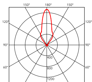
— C0 / C180 cd / 1000 lm ..... C90 / C270
